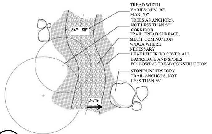
PLAN DETAIL: FRONTCOUNTRY TRAIL- TYP.
